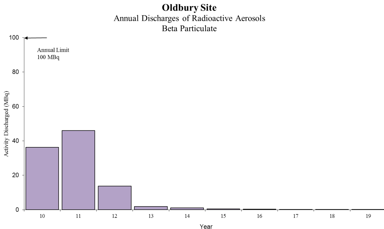
Fig 3.5 Oldbury Site, Annual Discharges of Radioactive Aerosols – Beta Particulate
