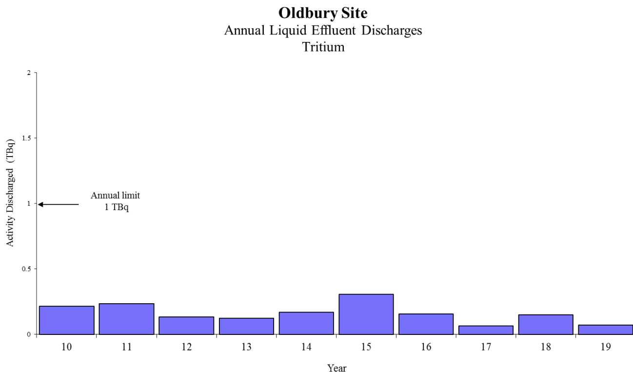
Fig 4.1 Oldbury Site, Annual Liquid Effluent Discharges of Tritium
