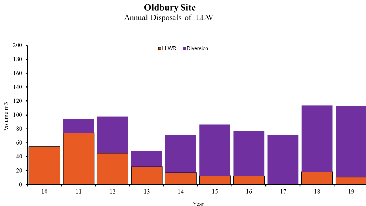
Fig 4.7 Oldbury Site, Annual Disposals of LLW
