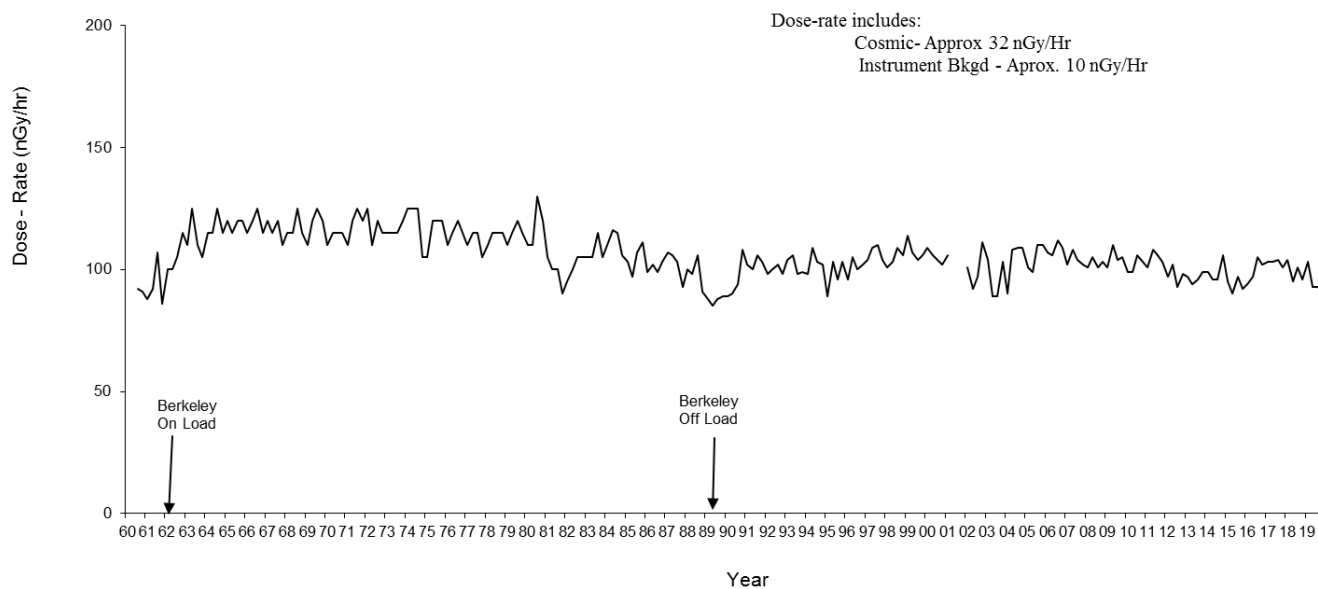
Fig 5.4 Berkeley Site, Radiation Dose rates at 0.5 – 1 km sites
