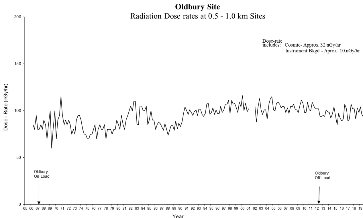
Fig 5.3 Oldbury Site, Radiation Dose rates at 0.5 – 1 km sites
